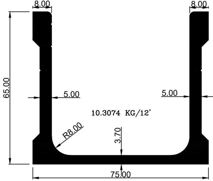
SECTION No.:—SE—903
