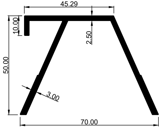
SECTION No.:--SE-838
