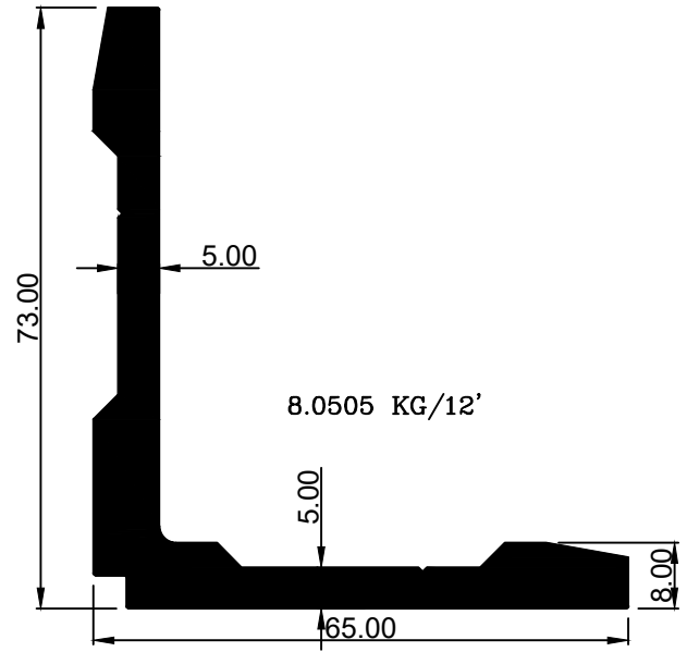
SECTION No.:—SE—901
